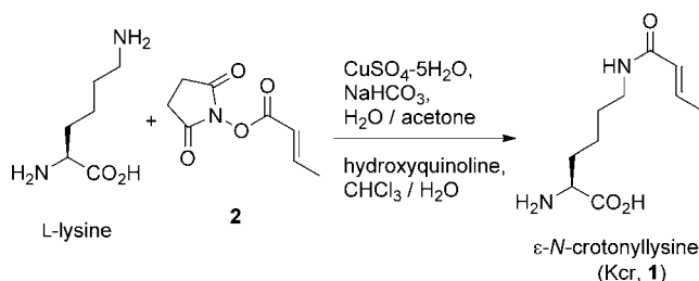
Scheme 1. Synthesis of \epsilon - N -crotonyllysine (Kcr, 1 ).
