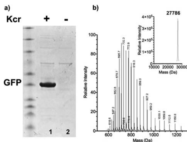
Figure 1. A) A mutant Mb-Pyl Kcr-RS/Pyl-tRNA pair selectively and efficiently incorporates Kcr in response to the TAG codon: GFP-Asp149TAG was expressed with or without 5 mM Kcr (lane 1 and lane 2, respectively) in the presence of an Mb-Pyl Kcr-RS/Pyl-tRNA pair. GFP mutant was purified by Ni-NTA affinity chromatography, analyzed by SDS-PAGE and stained with Coomassie Blue. B) ESI-MS analysis of purified mutant GFP; the peak corresponds to full-length GFP-Asp149Kcr-His 6 (expected: 27789, observed: 27786).
